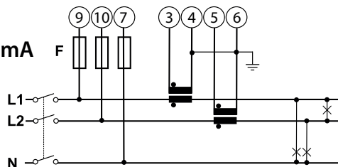
Connection from 2 TA
