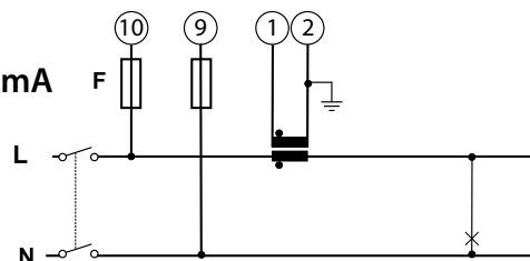
Connection from 1 TA
